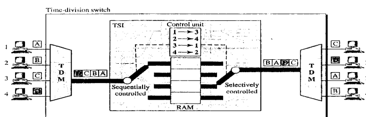
Figure 6.6 Time-slot interchange
