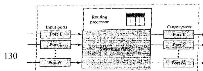
Figure 6.7 Packet switch components
