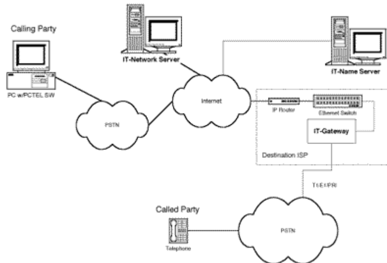
Figure 7. PC-to-Phone Connection
