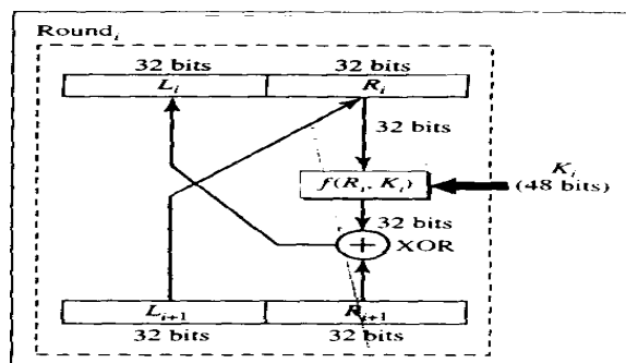
Figure 3.14 One round in DES ciphers
