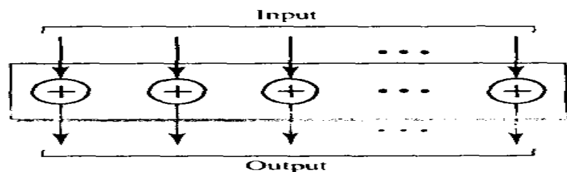
Figure 30.9 XOR cipher
