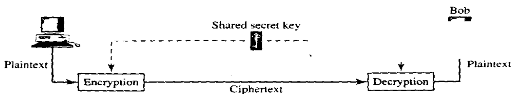
Figure 3.3 Symmetric-key cryptography
