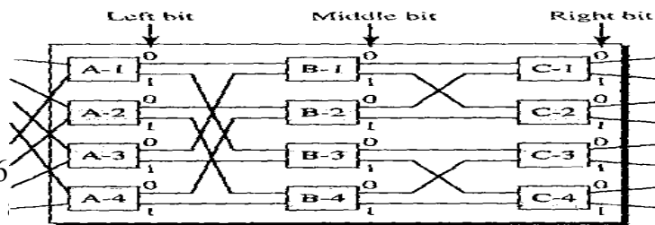
Figure 6.9 A banyan switch
