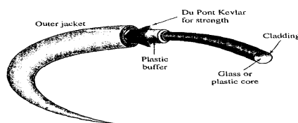
Figure 7.14 Fiber construction
