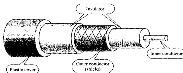
Figure 7.7 Coaxial cable
