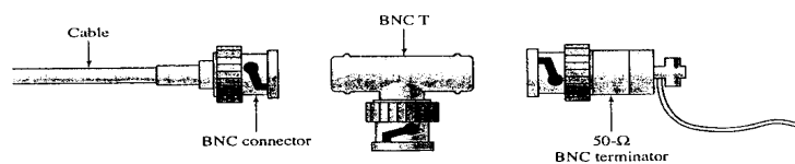
Figure 7.8 BNC connectors
