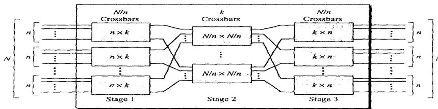
Figure 6.5 Multistage switch
