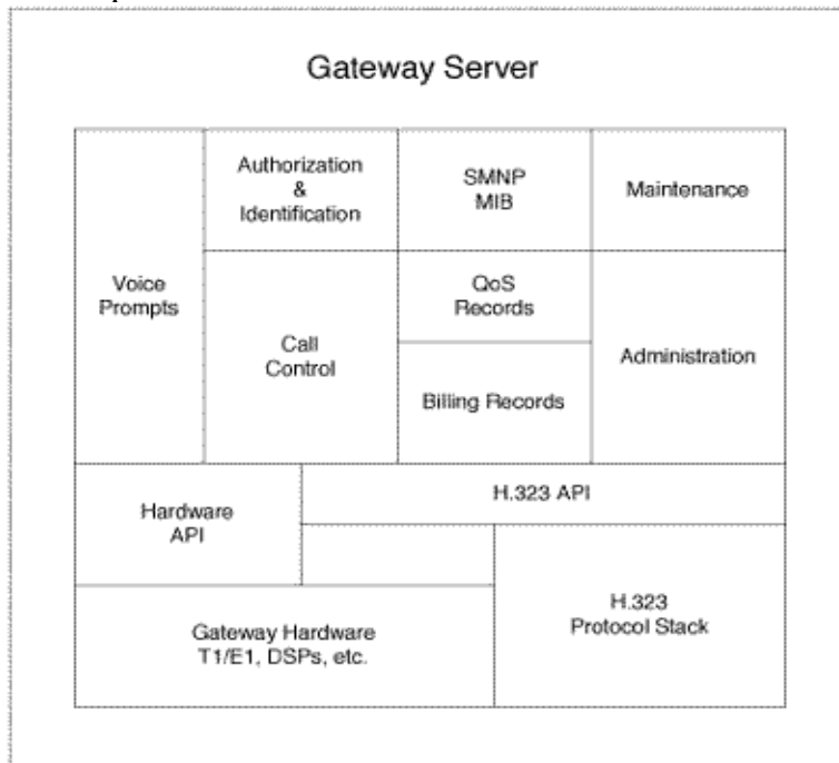
Figure 9. Internet Telephony
