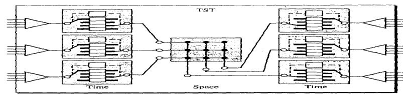
Figure 6.7 Time-space-time switch
